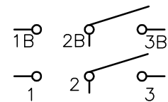
CIRCUIT: DPDT CONTACT CONFIGURATION
