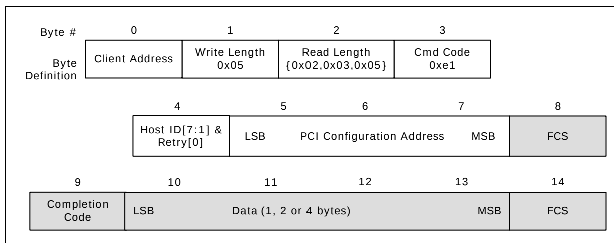
Figure 2-47. RdPCIDConfigLocal()
