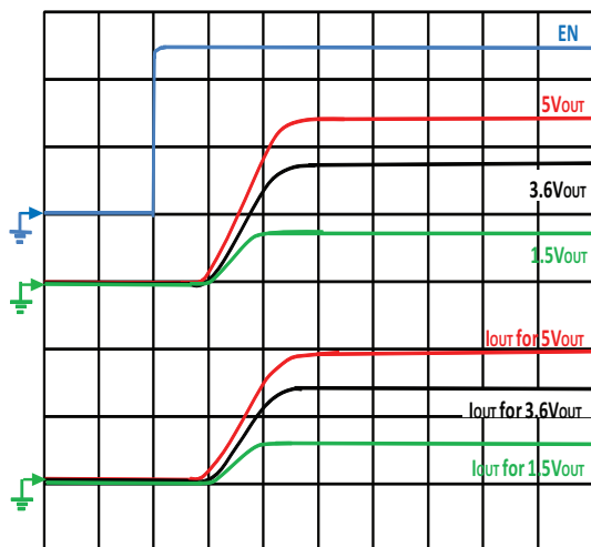
Figure 24 - Typical Turn-on Delay, Rise Time
