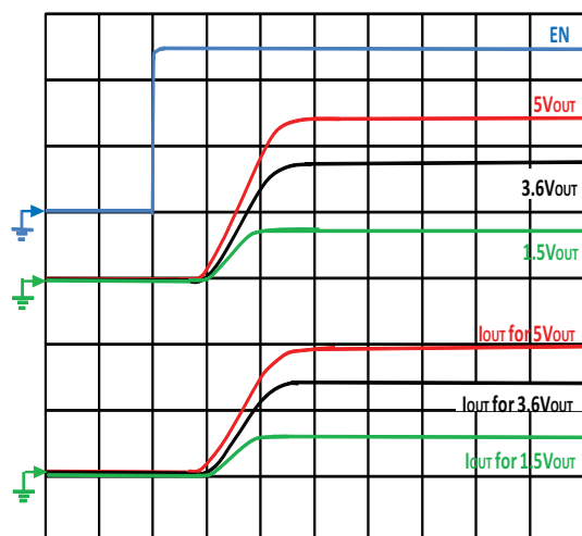
Figure 24 - Typical Turn-on Delay, Rise Time C_{OUT} = 200 \mu F , C_{IN} = 4.7 \mu F , R_{OUT} = 10 \Omega
