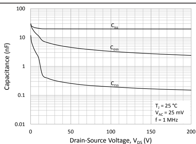
Figure 14. Typical Capacitances vs. Drain-Source Voltage (0 - 200 V)
