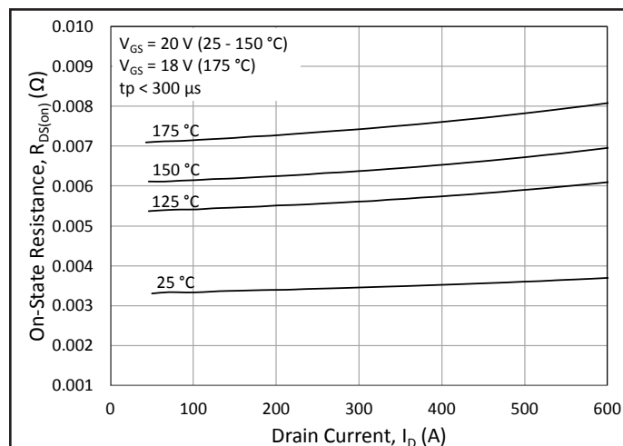
Figure 7. On-State Resistance vs. Drain Current for Various Temperatures
