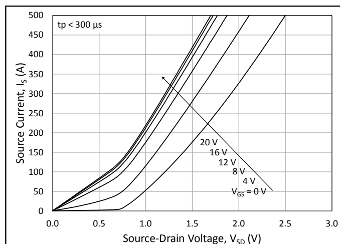
Figure 11. 3 rd Quadrant Characteristic at 150 °C
