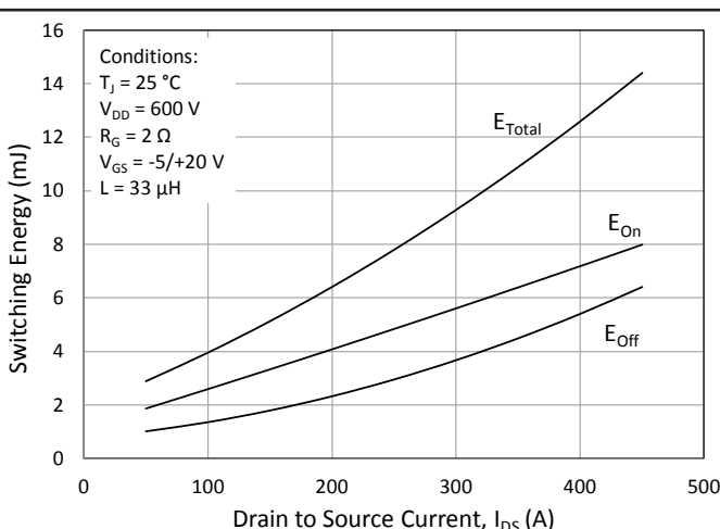
Figure 16. Inductive Switching Energy vs. Drain Current For V_{DD} = 600\text{ V} , R_G = 2\ \Omega
