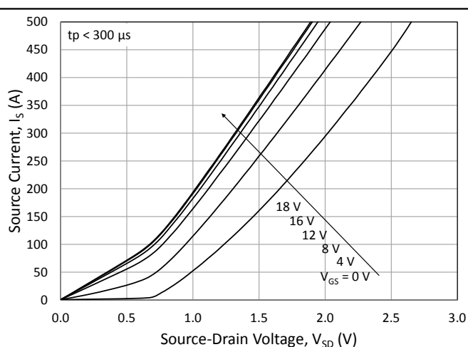
Figure 12. 3 rd Quadrant Characteristic at 175 °C
