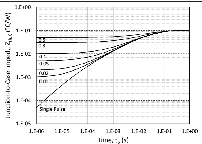
Figure 22. MOSFET Junction-to-Case Thermal Impedance
