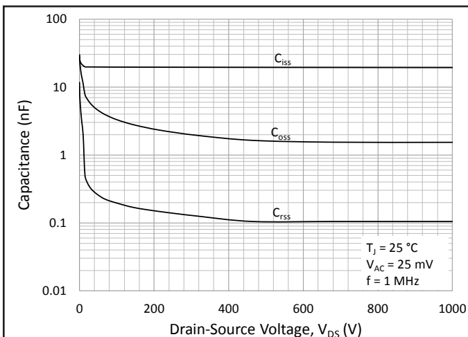
Figure 15. Typical Capacitances vs. Drain-Source Voltage (0 - 1 kV)
