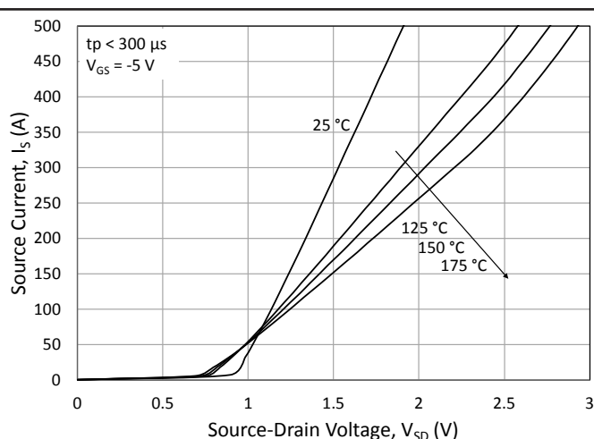
Figure 8. Antiparallel Diode Characteristic for Various Temperatures, V_{GS} = -5\text{ V}
