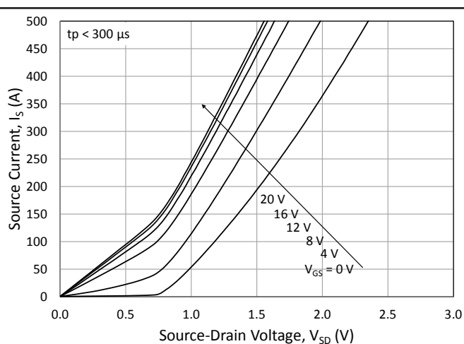
Figure 10. 3 rd Quadrant Characteristic at 125 °C
