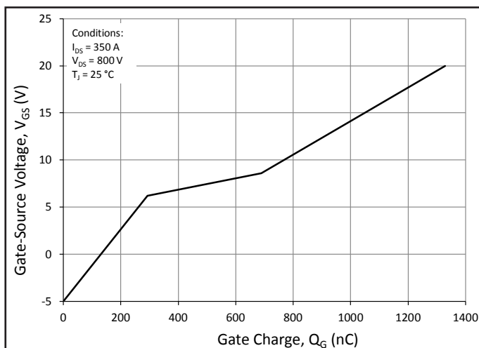
Figure 13. Scaled Gate Charge Characteristic
