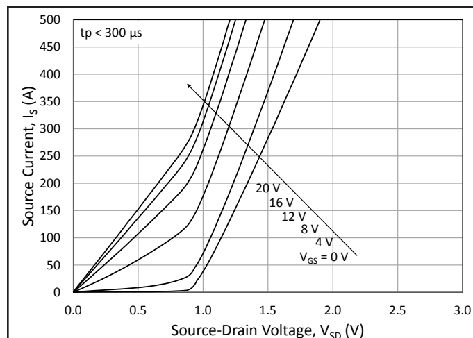
Figure 9. 3 rd Quadrant Characteristic at 25 °C
