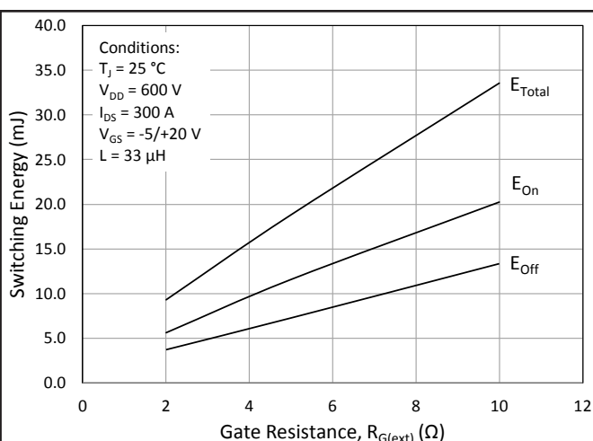
Figure 18. Inductive Switching Energy vs. External Gate Resistance, I_{DS} = 300\text{ A}
