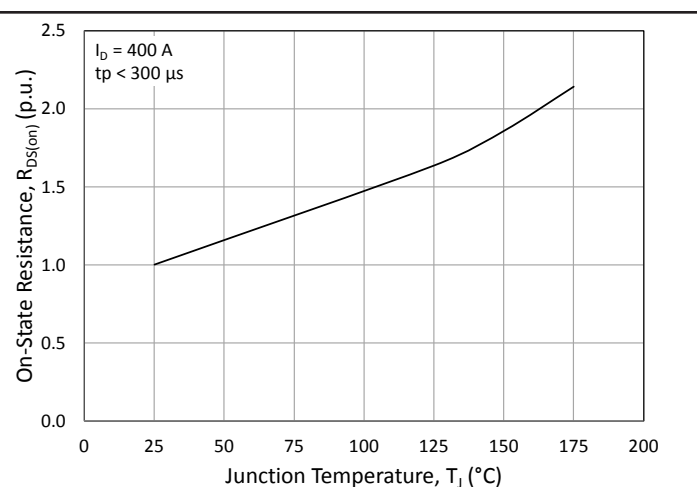
Figure 6. Normalized On-State Resistance vs. Temperature
