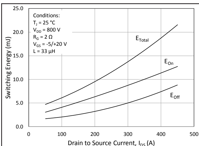
Figure 17. Inductive Switching Energy vs. Drain Current For V_{DD} = 800\text{ V} , R_G = 2\ \Omega
