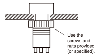
Screw Mounting
