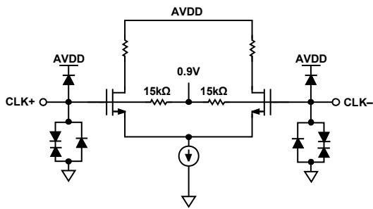
Figure 40. Equivalent Clock Input Circuit
