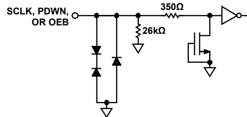
Figure 43. Equivalent SCLK, PDWN, or OEB Input Circuit
