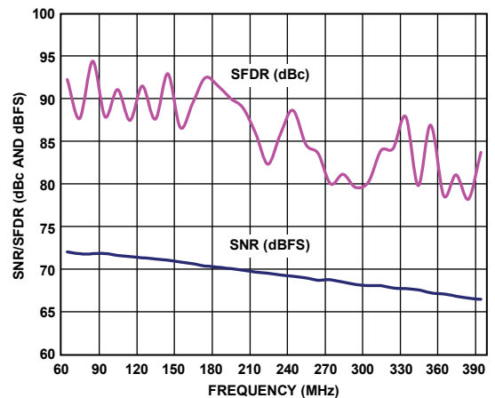
Figure 21. AD9643-210 Single-Tone SNR/SFDR vs. Input Frequency ( f_{IN} )
