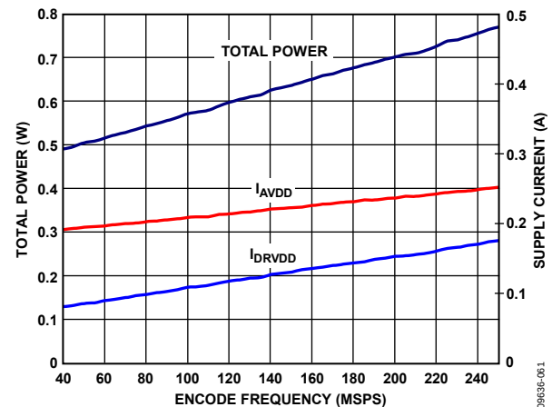
Figure 57. AD9643-250 Power and Current vs. Sample Rate
