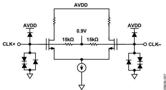
Figure 40. Equivalent Clock Input Circuit
