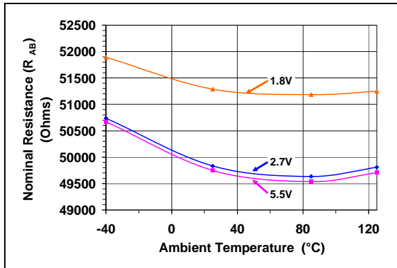
FIGURE 2-32: 50 kΩ – Nominal Resistance (Ω) vs. Ambient Temperature and V_{DD} .
