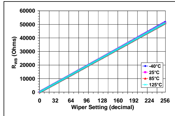
FIGURE 2-33: 50 kΩ – R_{WB} (Ω) vs. Wiper Setting and Ambient Temperature.
