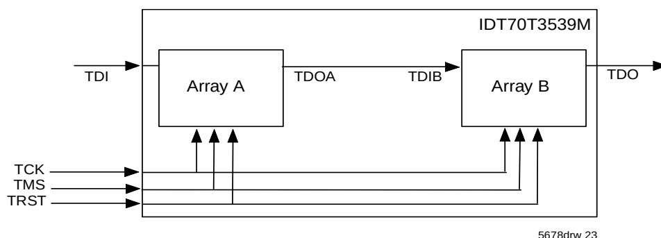
Figure 5. JTAG Configuration for IDT70T3539M
