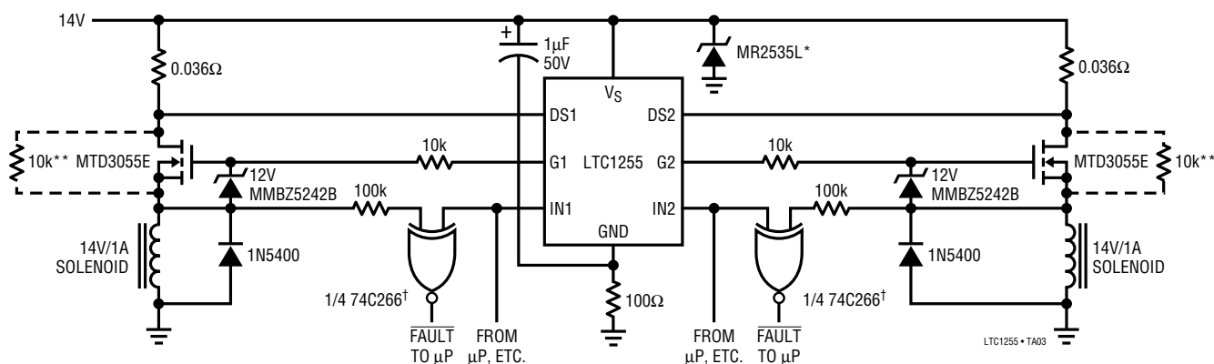
Dual Automotive High-Side Switch with Overvoltage Protection, XNOR Status and 12 \mu A Standby Current
