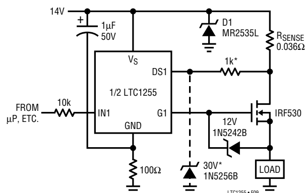
* OPTIONAL OVERVOLTAGE (30V) LATCH-OFF COMPONENTS
