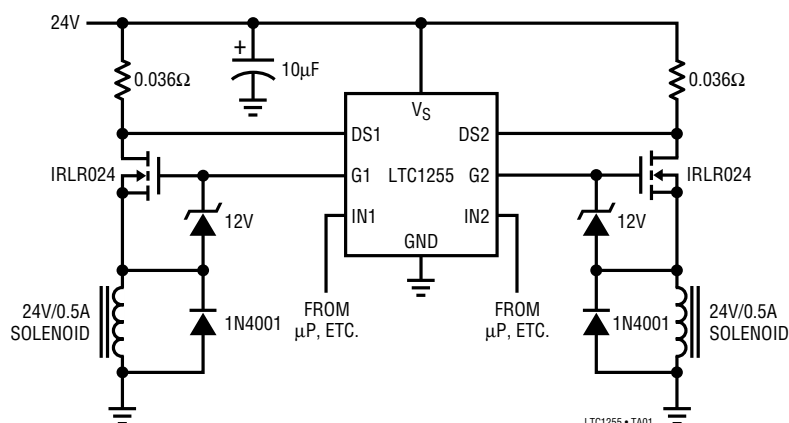
Dual 24V High-Side Switch with Overcurrent Protection
