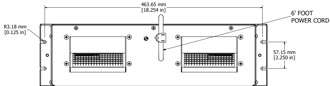
ASSEMBLY - VIEW FROM BACK
