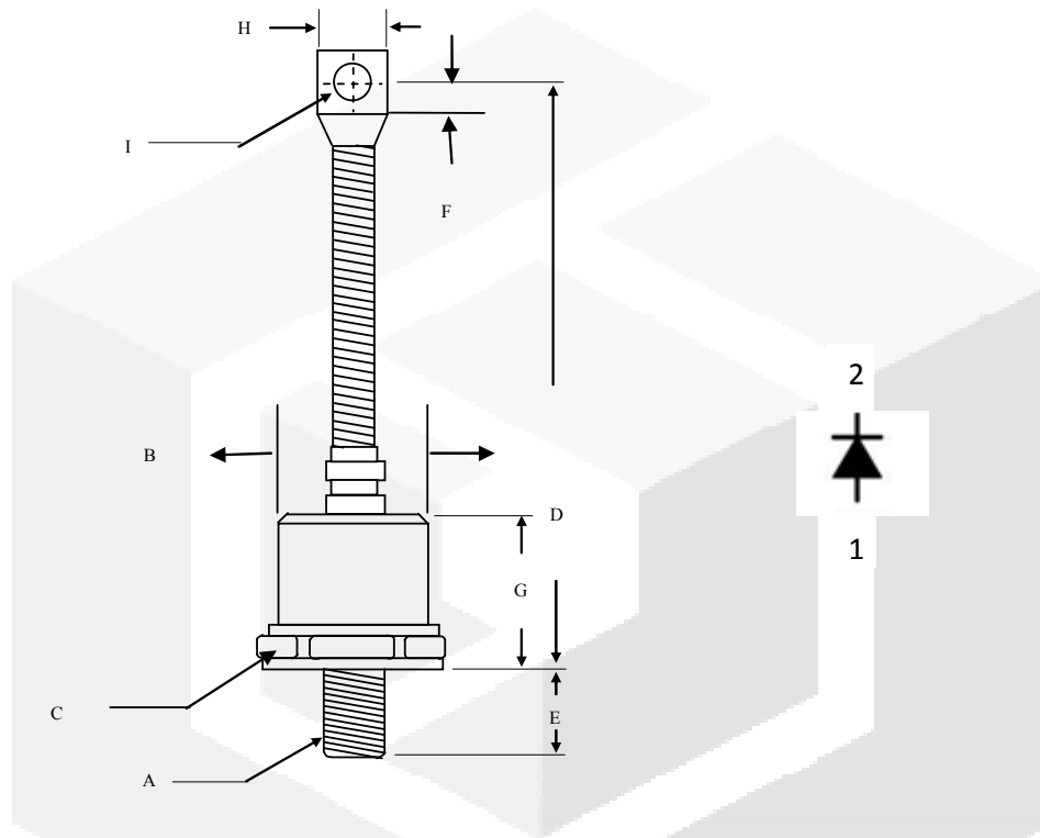
DO-9 (DO-205AB)
