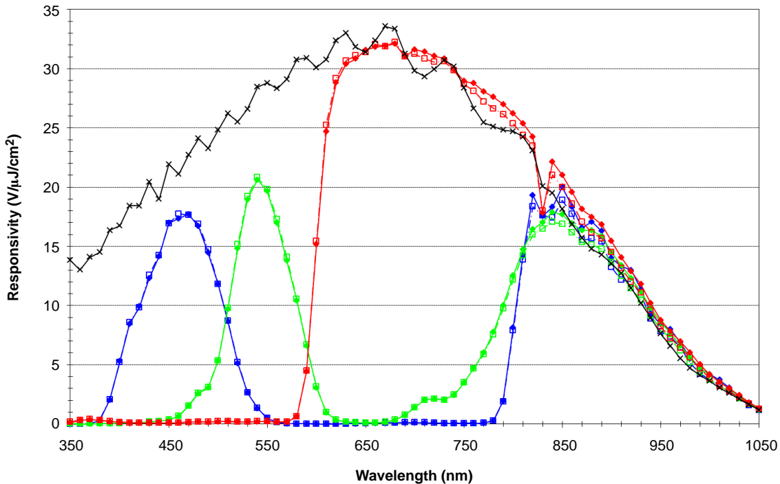
Figure 12. Typical Responsivity
