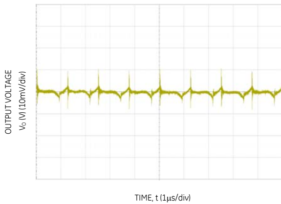
Figure 21. Typical output ripple and noise ( C_o = 6 \times 47\mu F ceramic, V_{IN} = 12V , I_o = I_{o,max} ).
