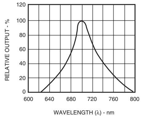
Fig. 2 SPECTRAL RESPONSE
