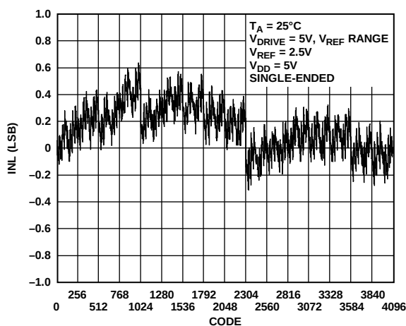
Figure 10. ADC INL Single-Ended, V_{REF} Range
