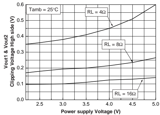
Figure 36. Clipping voltage vs. power supply voltage and load resistor T_{amb} = 25 °C
