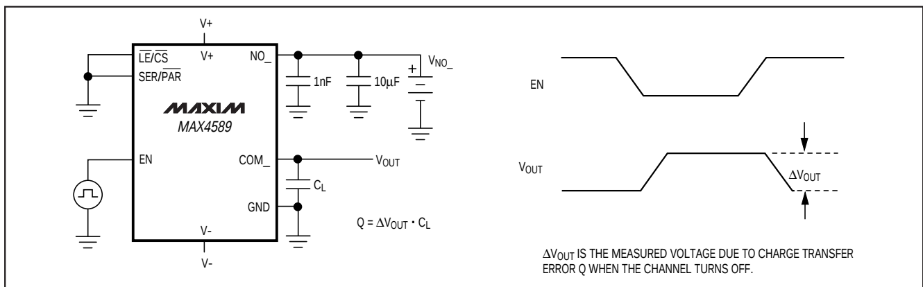
Figure 3. Charge Injection
