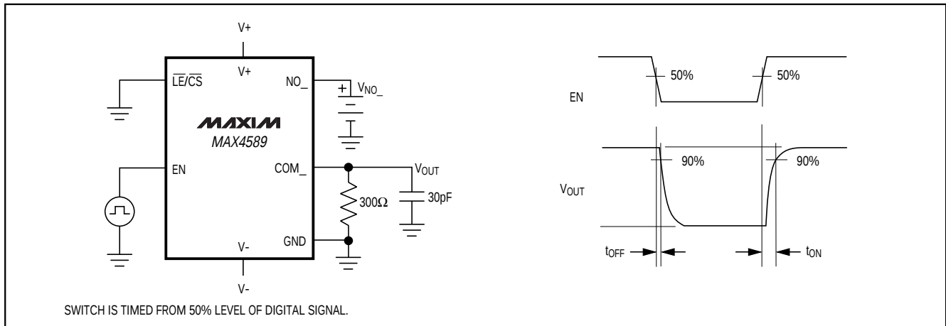
Figure 1. Turn-On/Turn-Off Time
