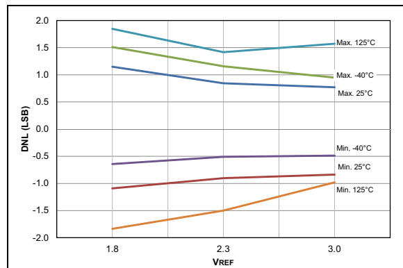
FIGURE 37-84: ADC 10-bit Mode, Single-Ended DNL, V_{DD} = 3.0V , T_{AD} = 1\text{ }\mu S .
