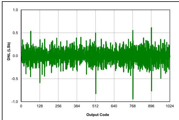
FIGURE 37-79: ADC 10-bit Mode, Single-Ended DNL, V_{DD} = 3.0V , T_{AD} = 4\text{ }\mu S , 25^\circ C .
