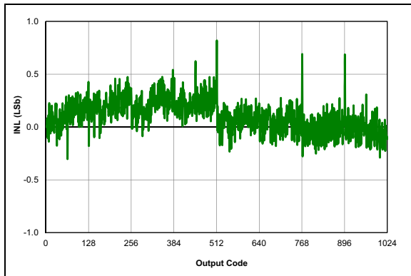
FIGURE 37-81: ADC 10-bit Mode, Single-Ended INL, V_{DD} = 3.0V , T_{AD} = 4\text{ }\mu S , 25^\circ C .
