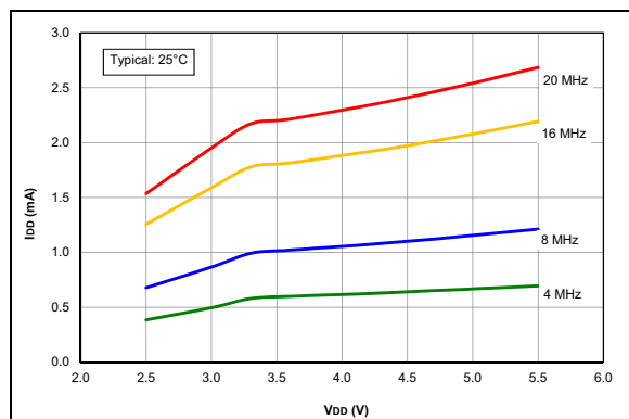
FIGURE 37-29: I_{DD} Typical, HS Oscillator, 25^\circ\text{C} , PIC16F1777/8/9 Only.
