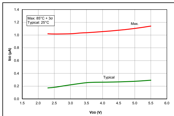
FIGURE 37-49: I_{D} , ADC Non-Converting, PIC16F1777/8/9 Only.
