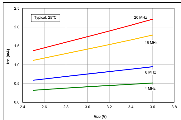
FIGURE 37-27: I_{DD} Typical, HS Oscillator, 25^\circ\text{C} , PIC16LF1777/8/9 Only.
