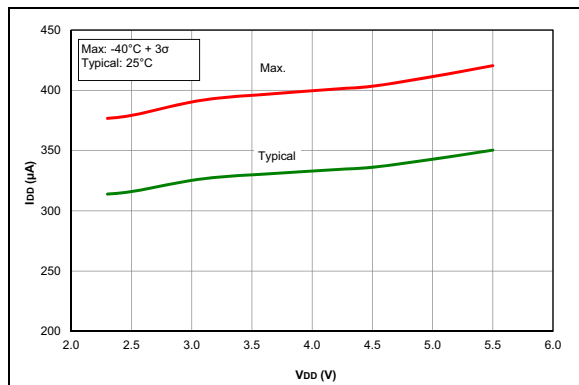
FIGURE 37-51: I_{D} , Comparator, NP Mode ( V_{REGPM} = 0 ), PIC16F1777/8/9 Only.
