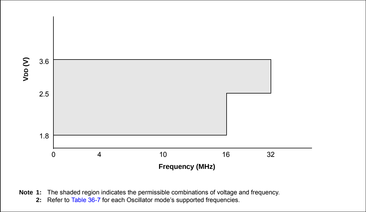
FIGURE 36-2: VOLTAGE FREQUENCY GRAPH, -40°C ≤ TA ≤ +125°C, PIC16LF1777/8/9 ONLY
