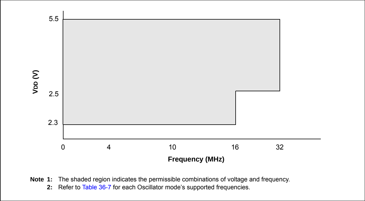
FIGURE 36-1: VOLTAGE FREQUENCY GRAPH, -40°C ≤ TA ≤ +125°C, PIC16F1777/8/9 ONLY
