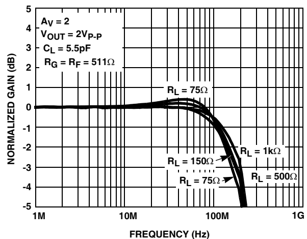
FIGURE 4. LARGE SIGNAL GAIN vs FREQUENCY vs R_L
