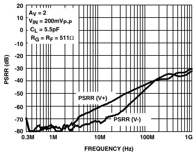
FIGURE 9. PSRR CHANNELS
