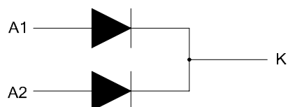
Figure 3. Internal Structure of MBR20200C
