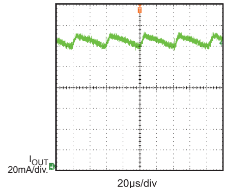
Output-Current Ripple
