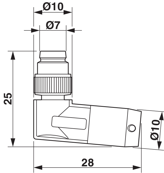
Dimensioned drawing
