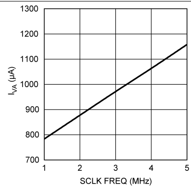
Figure 28. V_A Current vs. SCLK Frequency
