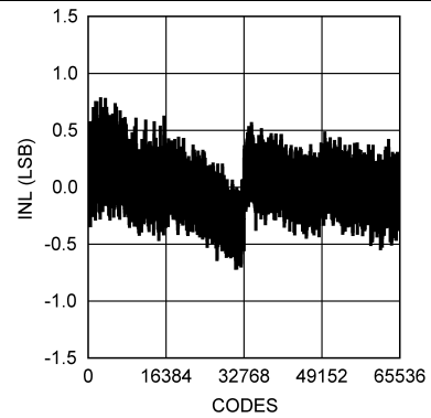
Figure 8. INL - 250 kSPS
