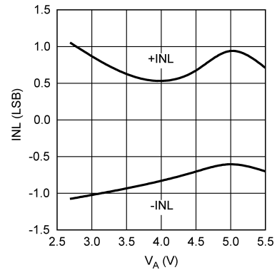
Figure 10. INL vs. V_A
