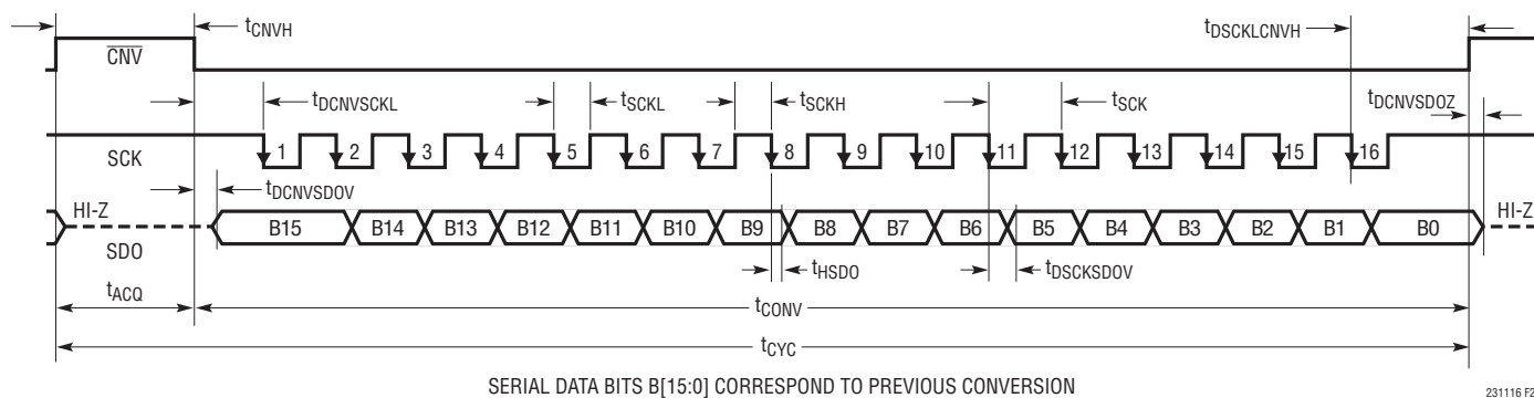
Figure 21. LTC2311-16 Timing Diagram, CMOS, LVDS I/O Modes
