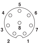
Pin assignment M12 socket, 8-pos., A-coded, view female side
