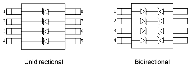
SCHEMATIC
