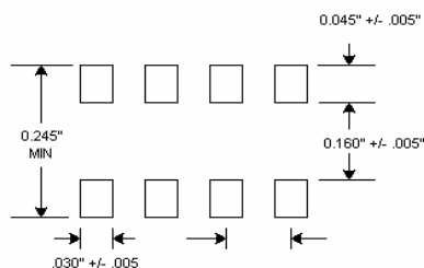
PAD LAYOUT
