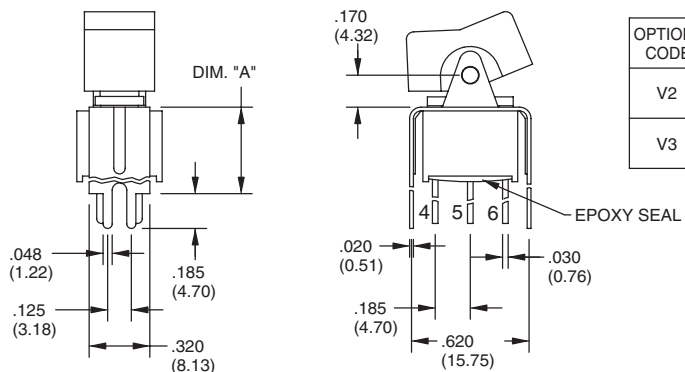
DPDT
