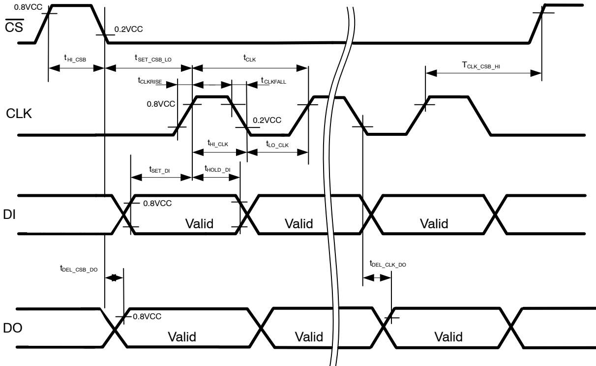
Figure 3. SPI Timing
