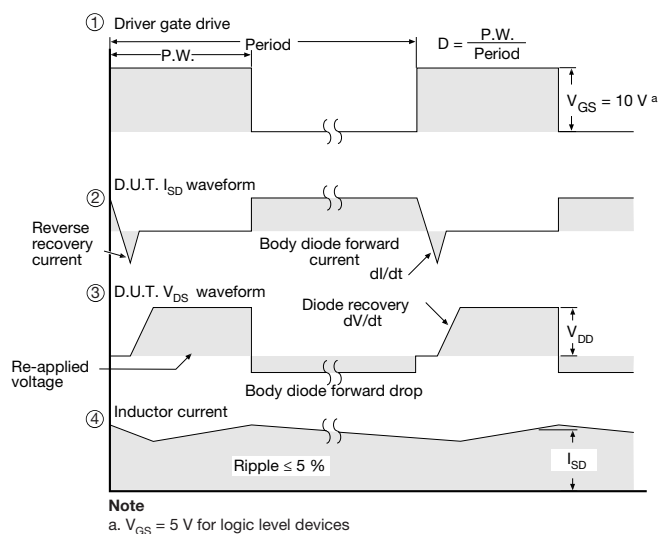
Fig. 20 - For N-Channel
