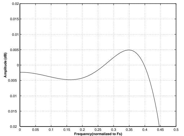
Figure 32. DAC Double Speed (fast) Passband Ripple
