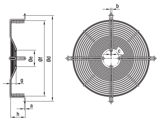
Basket guard grille for K series axial fans
