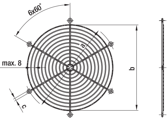
Guard grilles (e.g. for axial fans)
