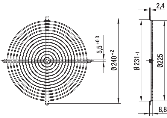
Guard grille for diagonal fan (outlet side mounting)
