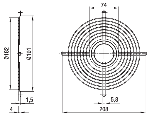
Guard grille for diagonal fan
