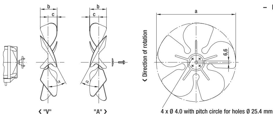
Axial impeller for Q-motors and energy-saving motors (ESM)
