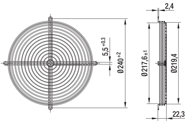
Guard grille for diagonal fan (inlet side mounting)
