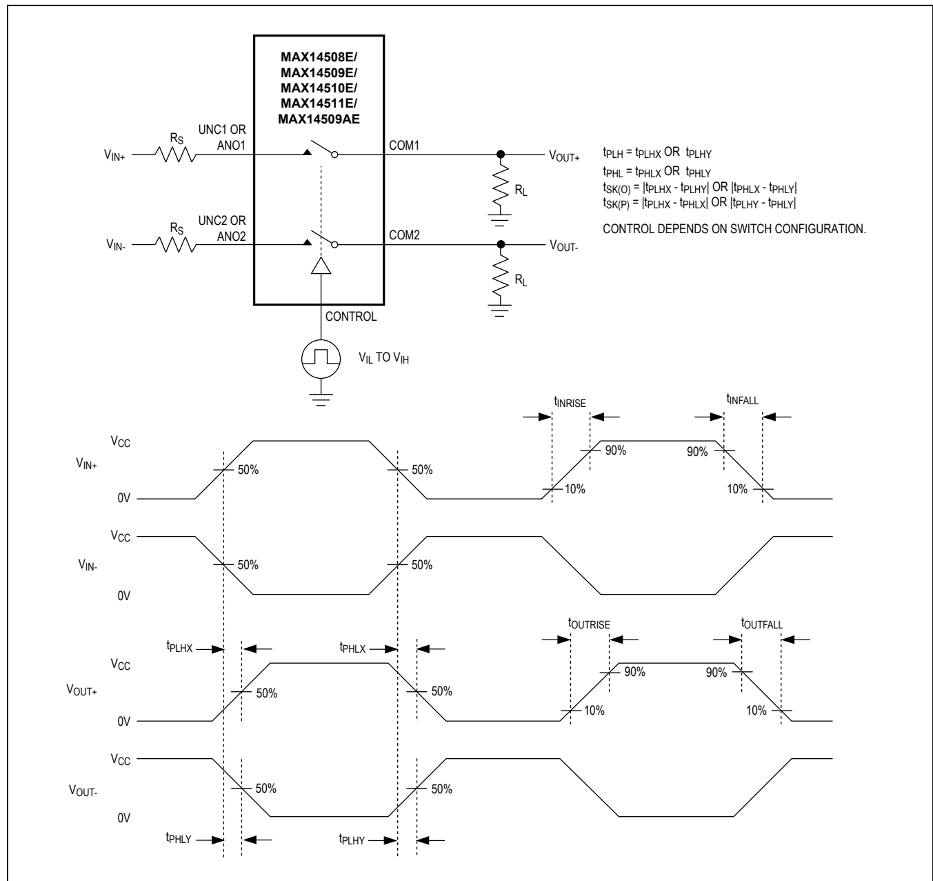
Figure 3. Output Skew
