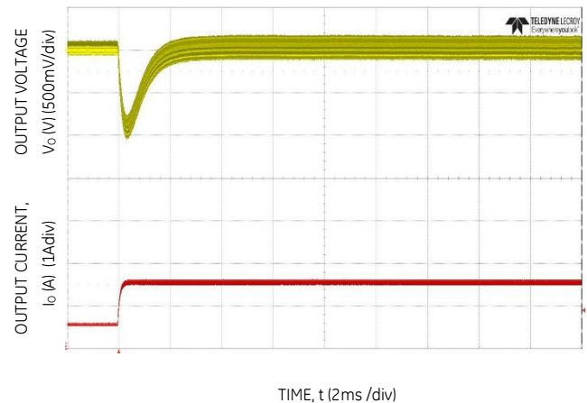
Figure 10. Transient Response to Dynamic Load Change from 0.6 to 1.6A at 12Vin, C out =10x4.7μF, C Tune =560pF, R Tune =40.2k
