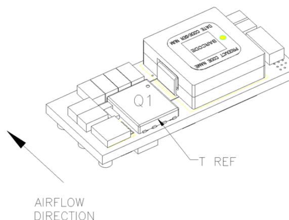
Figure 34. Preferred airflow direction and location of hot-spot of the module ( T_{ref} ).
