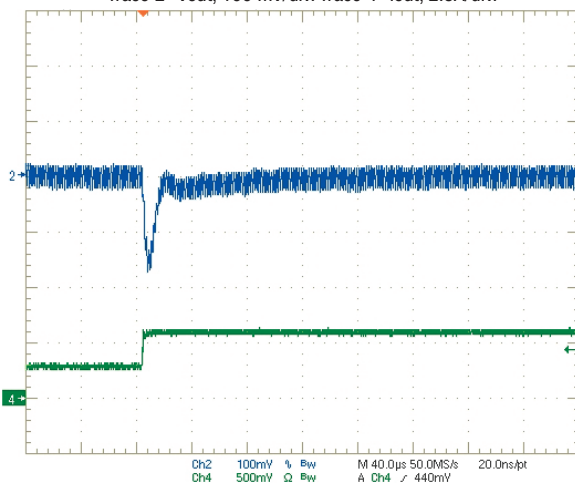
Step Load Transient Response (Vin=12V, Vout=2.5V, Load=0, Iout=1.5A to 3A) Trace 2=Vout, 100 mV/div. Trace 4=Iout, 2.5A/div.
