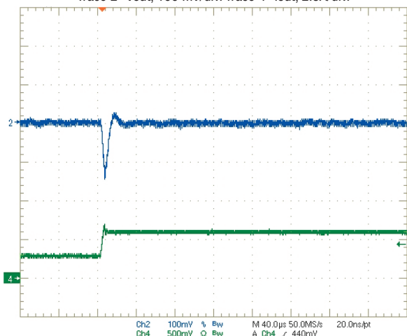
Step Load Transient Response (Vin=12V, Vout=0.591V, Cload=0, Iout=1.5A to 3A) Trace 2=Vout, 100 mV/div. Trace 4=Iout, 2.5A/div.
