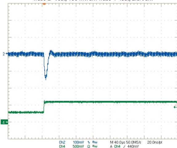
Step Load Transient Response (Vin=12V, Vout=1.2V, Cload=0, Iout=1.5A to 3A) Trace 2=Vout, 100 mV/div. Trace 4=Iout, 2.5A/div.
