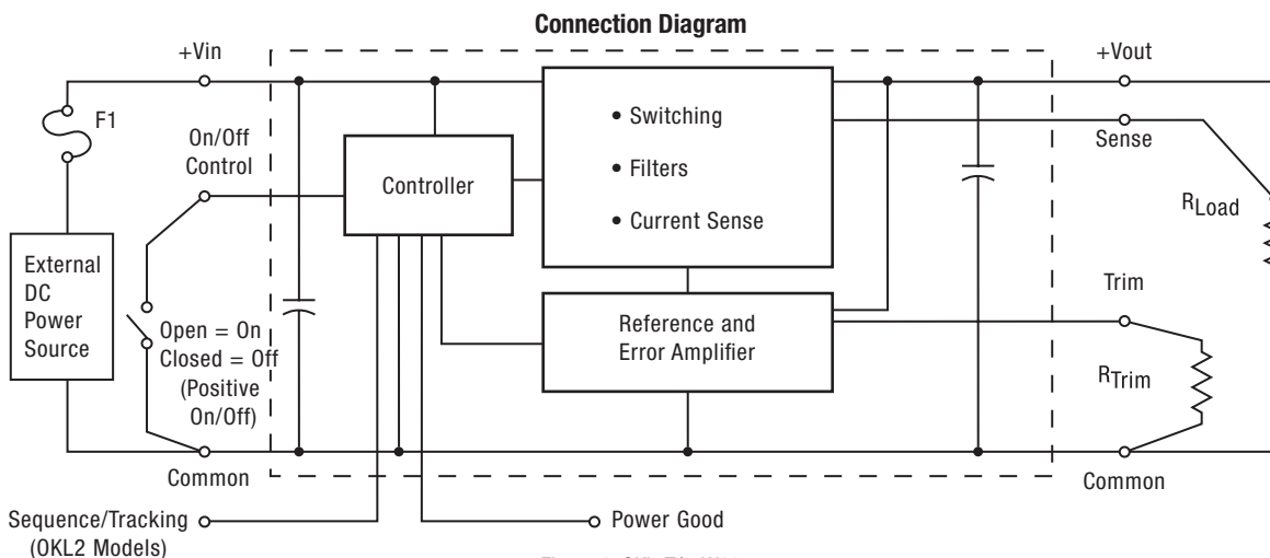
Figure 1. OKL-T/3-W12
