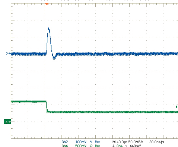
Step Load Transient Response (Vin=12V, Vout=0.591V, Cload=0, Iout=3A to 1.5A) Trace 2=Vout, 100 mV/div. Trace 4=Iout, 2.5A/div.
