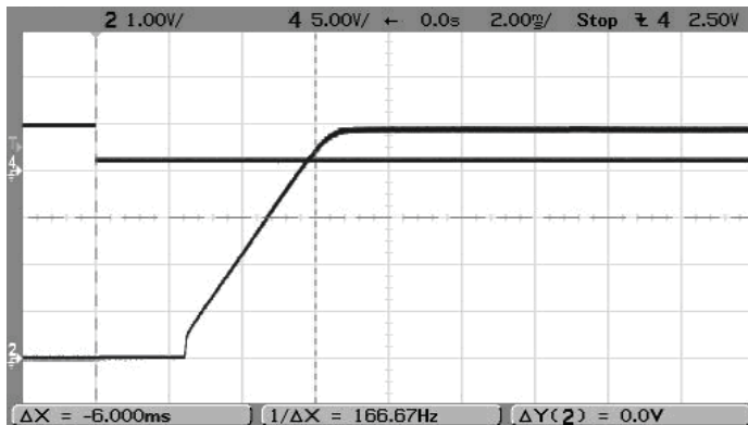
On/Off Enable Startup Delay (Vin=12V, Vout=5.0V, Iout=3A, Cload=0) Trace 4=Enable In, Trace2=Vout
