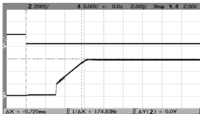
On/Off Enable Startup Delay (Vin=12V, Vout=0.591V, Iout=3A, Cload=0) Trace 4=Enable In, Trace2=Vout
