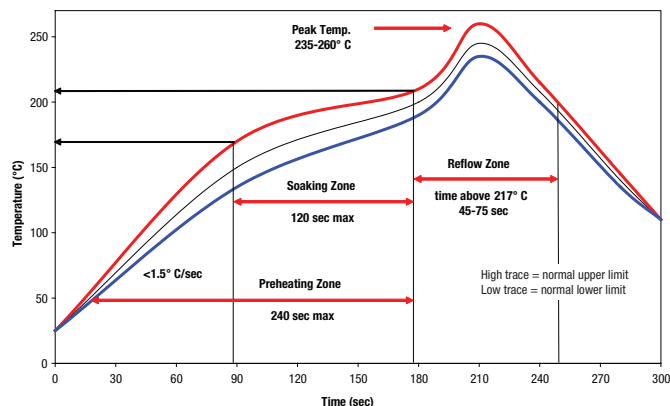
Recommended Lead-free Solder Reflow Profile
