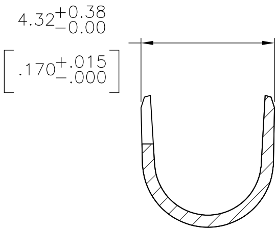
SECTION X-X
