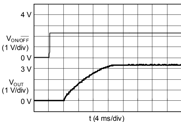
(6) S-8540A18FN ( V_{\text{IN}} : 10 \text{ V} )
