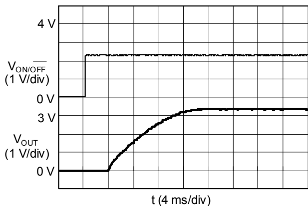
(3) S-8540C33FN ( V_{\text{IN}} : 4.95 \text{ V} )
