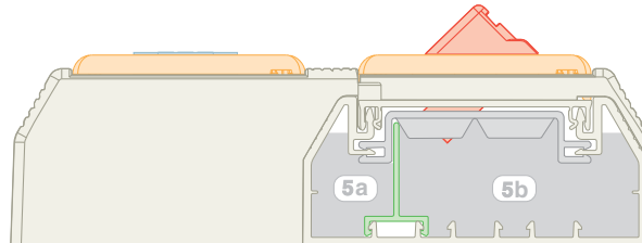
Cable fill #3: Data only using vertical sloped screw-on communication faceplates.
