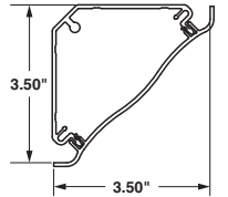
COVE RACEWAY Internal Area = 5.40 Sq. In. (3484 Sq. mm)
