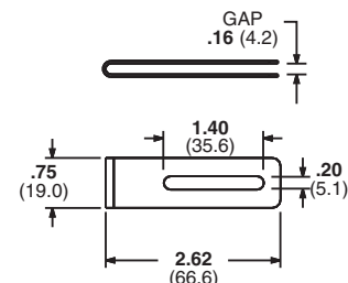
Bonding clip (for use with wiring duct).
