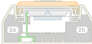
Cable fill #2: Power and data using 3-sided hanging box and device bracket.
