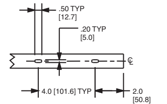
Mounting Hole Dimensions For .5", .75", 1", and 1.5" wide duct.
