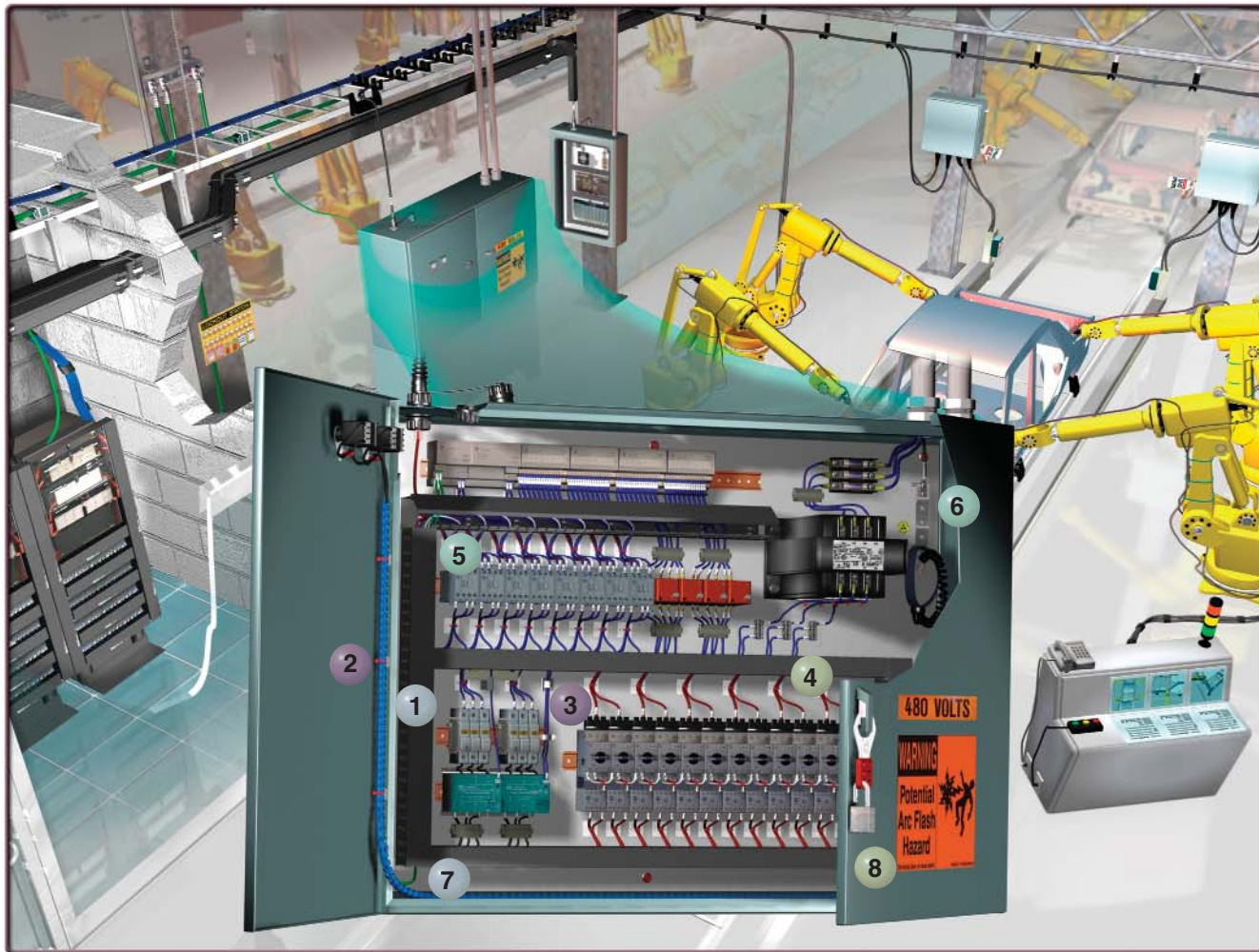
1 Wiring Duct
