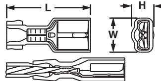
Cross section of DiscoGrip™ Crimp showing insulation crimp of the wire insulation.
