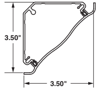
COVE RACEWAY Internal Area = 5.40 Sq. In. (3484 Sq. mm)
