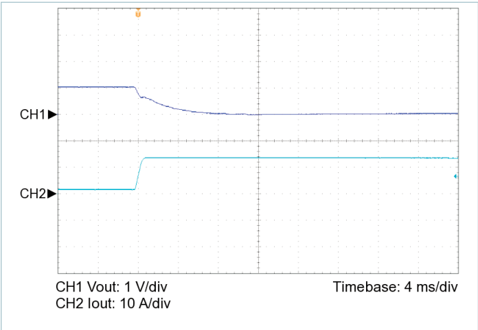
Figure 8 — 10% to 100% load transient response, V_{IN} = 48\text{ V} , nominal trim, C_{OUT\_EXT} = 1000\text{ }\mu\text{F}
