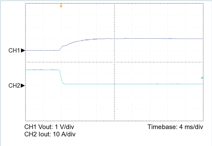
Figure 7 — 100% to 10% load transient response, V_{IN} = 48\text{ V} , nominal trim, C_{OUT\_EXT} = 1000\text{ }\mu\text{F}
